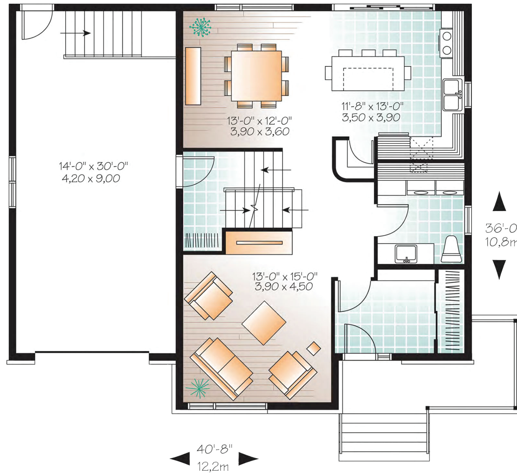
MAIN FLOOR PLAN PLANCHER PRINCIPAL
